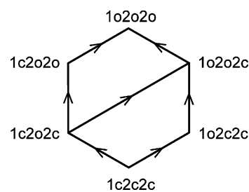
Figure 2. Graph of isomerization pathways for 122 . Net photochemical isomerization under the influence of UV light occurs in the direction of the arrows. Thermal isomerization and photoisomerization promoted by visible light occurs in the opposite direction.
