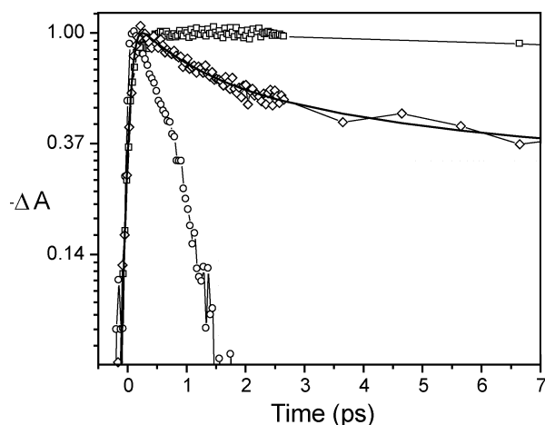
Figure 6. Transient absorption kinetics at 720 nm following excitation with a 585 nm, ca. 100 fs, laser pulse during constant illumination of the sample at 366 nm. Data for model compounds 3 (□) and 4 (○) and triad 122 (◇) are shown. The figure shows the negative of the absorbance change on a natural logarithm scale for the first 7 ps of the observation period. The solid line is a multiexponential fit to the data for 122 , as discussed in the text. The \Delta A values have been normalized for ease in comparison of the kinetics; the actual values are between 0.03 and -0.03 .
