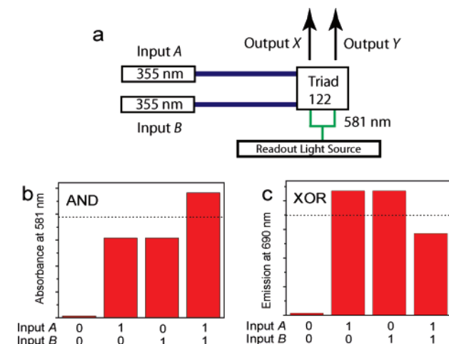
Figure 3. (a) Schematic diagram of the half-adder. (b) Actual performance of the AND gate function under the application of various combinations of inputs. (c) Performance of the XOR gate function. For signal-to-noise ratios in the absorption and emission readout processes, and for reproducibility of the data from one experiment to another, see Figures 7 and 8, respectively.
