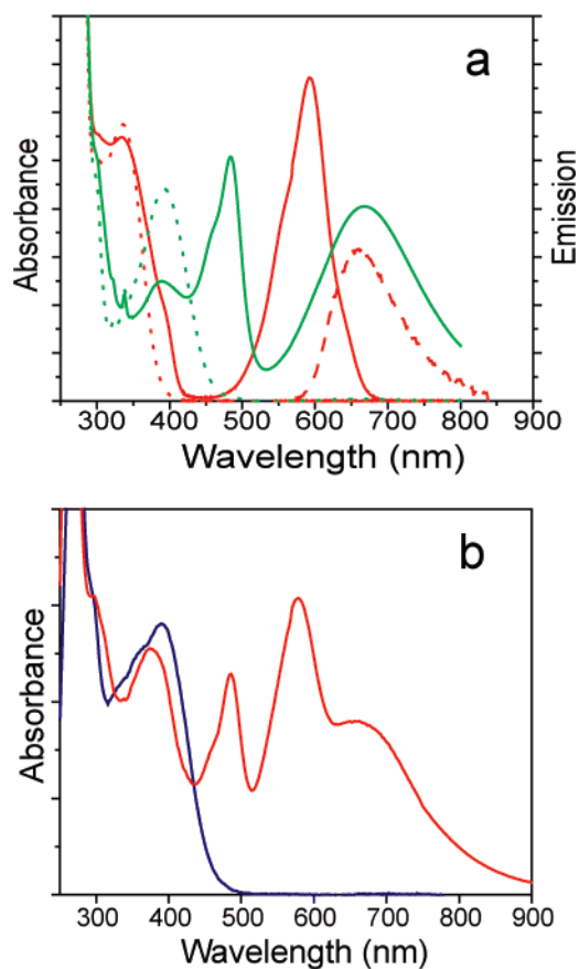
Figure 5. (a) Absorption spectra of 3c (red dots), a photostationary distribution containing mainly 3o (red line), 4c (green dots), a photostationary distribution containing mainly 4o (green line), and emission spectrum of 3o (red dashes). (b) Absorption spectra of 1c2c2c (blue line), and the same solution after irradiation at 355 nm to generate a photostationary distribution rich in the open forms of the triad (red line).
