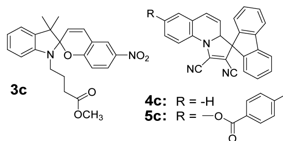
Figure 4. Structures of the closed, spiro forms of model spiroopyran 3c and model quinoline-derived dihydroindolizines 4c and 5c . The structures of the open forms ( 3o , 4o , 5o ) are analogous to those of the corresponding structures in 1o and 2o (Figure 1).
