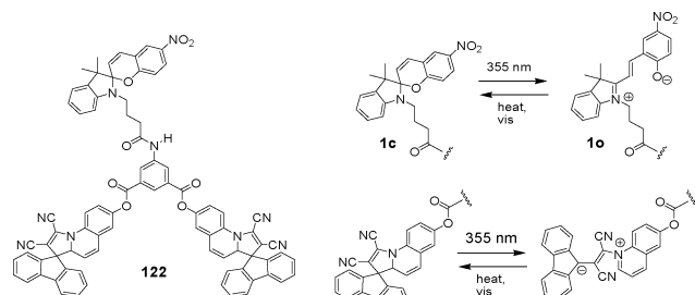
Figure 1. Structure of triad 122 and isomerization of the spiro-spiro-pyrans ( 1 ) and quinoline-derived dihydroindolizine ( 2 ) photochromes.
