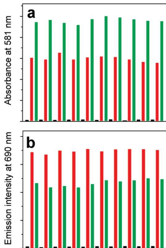
Figure 8. Cycling of the triad. (a) Absorbance at 581 nm following reset ( 580 \leq \lambda \leq 900 nm, ca. 50 \text{ mW/cm}^2 , 10 min) (black), irradiation with one input (355 nm laser pulses at 5 Hz, 14 mW average power, 6.5 s) (red), and irradiation with both inputs (355 nm laser pulses at 10 Hz, 28 mW average power, 6.5 s) (green). (b) Emission at 690 nm (581 nm excitation) following the same sequence of irradiations.
