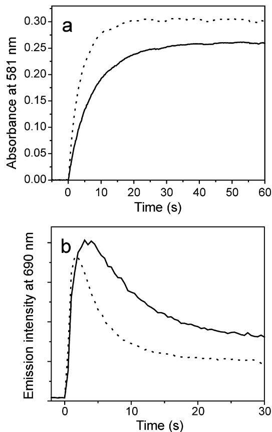
Figure 7. (a) Absorbance of a solution of 122 in 2-methyltetrahydrofuran at 581 nm as a function of irradiation time with 355 nm laser pulses having a repetition rate of 5 Hz (—) or 10 Hz (---). (b) Fluorescence of a solution of 122 in 2-methyltetrahydrofuran at 690 nm ( \lambda_{\text{ex}} = 581 nm) as a function of irradiation time with 355 nm laser pulses having a repetition rate of 5 Hz (—) or 10 Hz (---).
